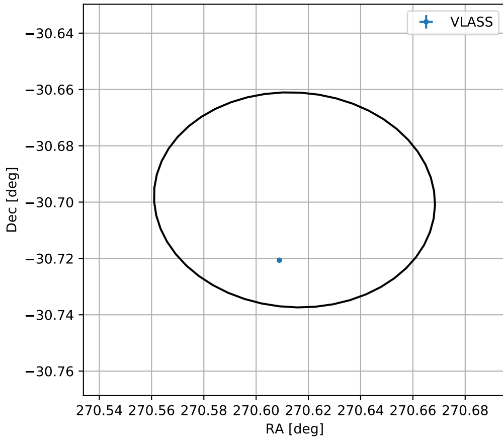
4FGL J1802.4-3041
