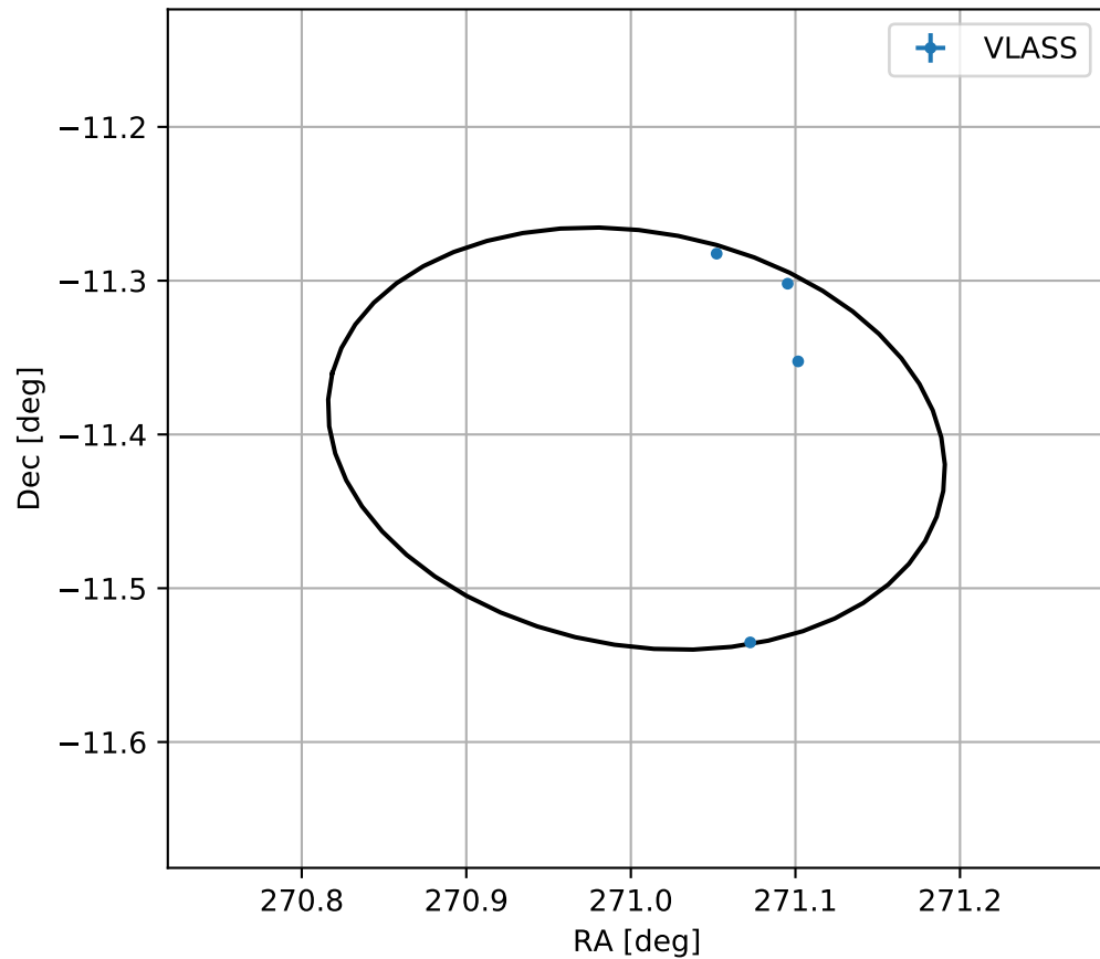
4FGL J1804.0-1124
