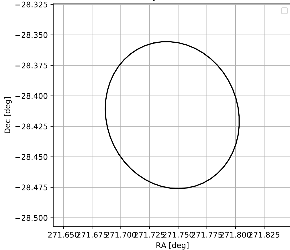
4FGL J1806.9-2824
