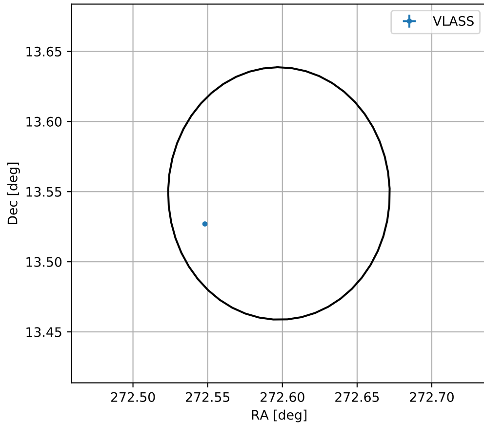
4FGL J1810.3+1332
