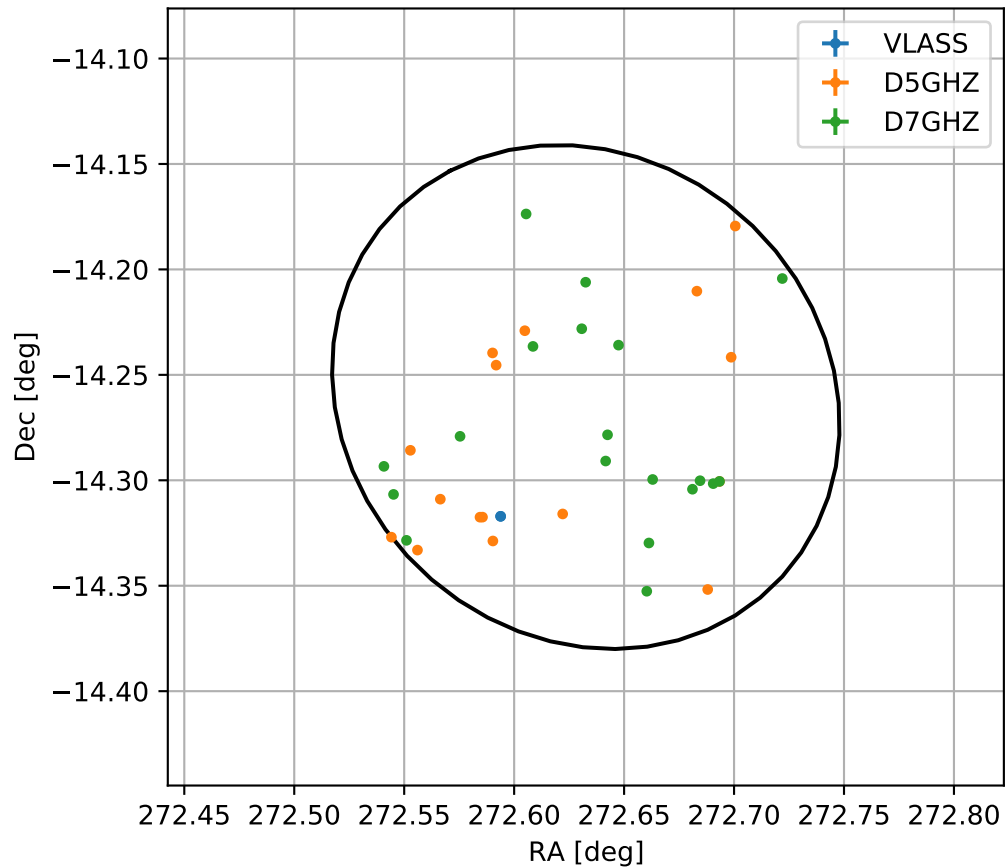
4FGL J1810.5-1415
