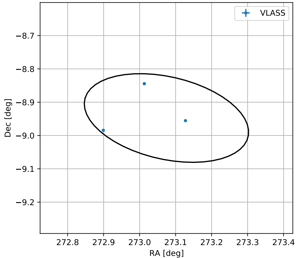
4FGL J1812.2-0856
