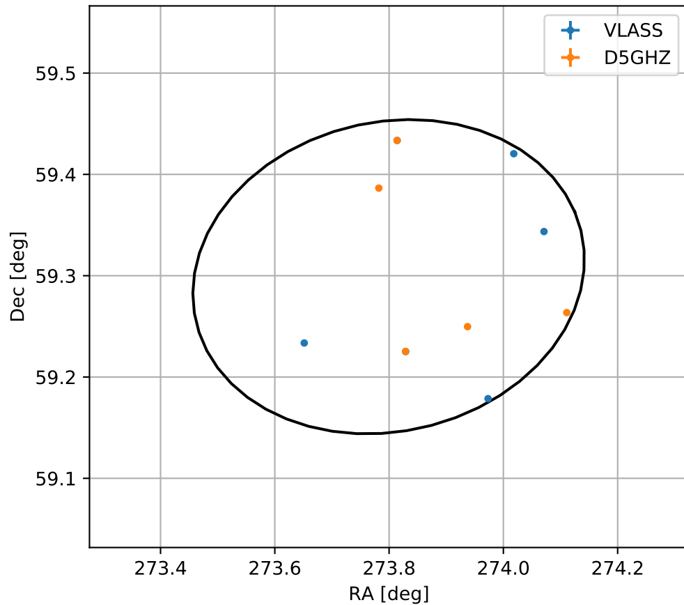
4FGL J1815.1+5917
