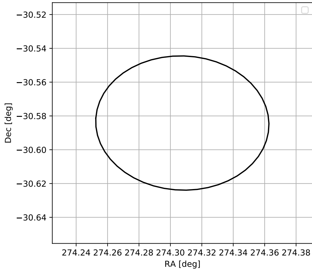
4FGL J1817.2-3035
