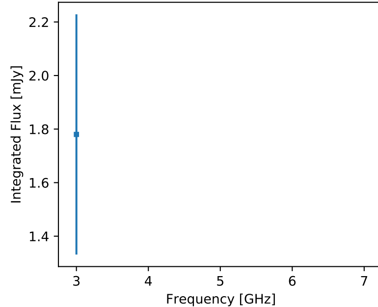
F357 J181705.83-103124.4 (unr)
