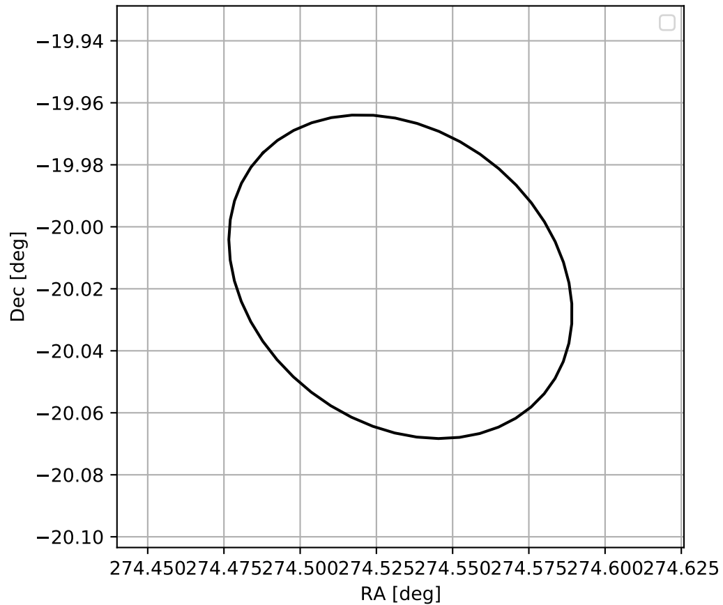
4FGL J1818.1-2000
