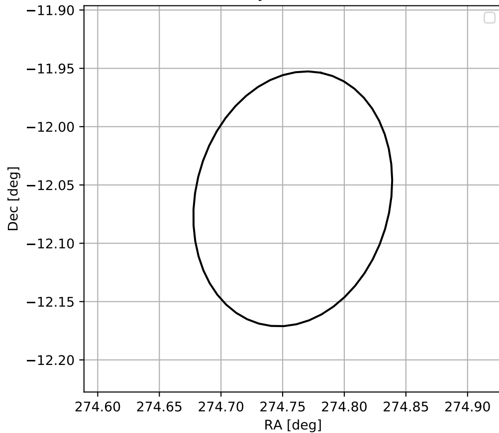
4FGL J1819.0-1203
