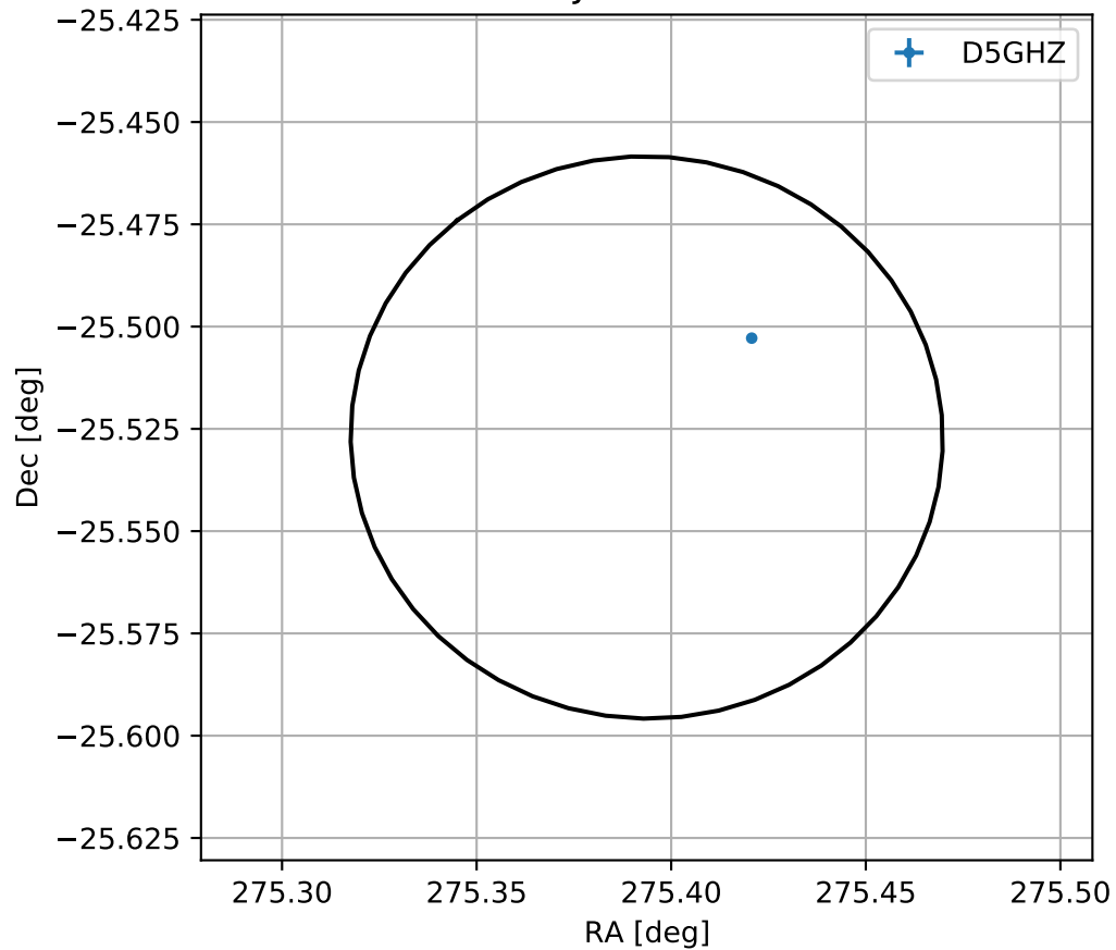
4FGL J1821.5-2531
