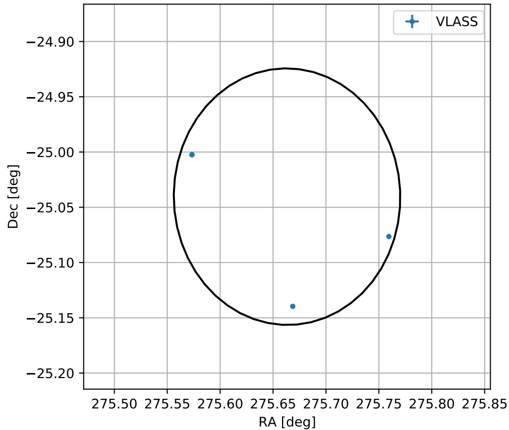
4FGL J1822.6-2502
