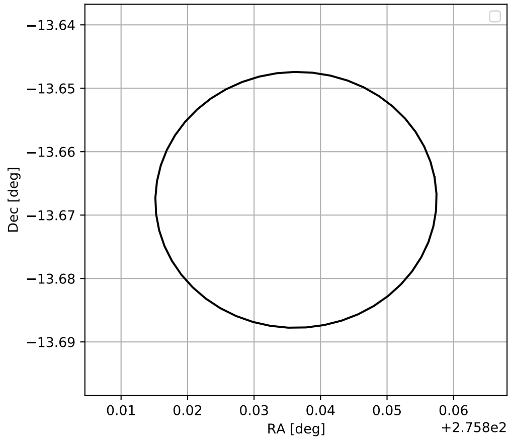
4FGL J1823.3-1340
