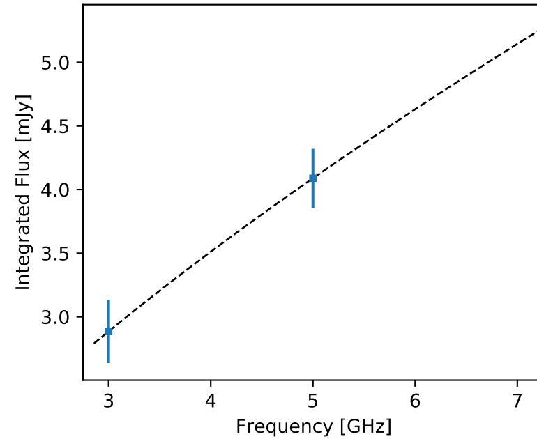
F357 J182947.95-254701.6 (unr)
