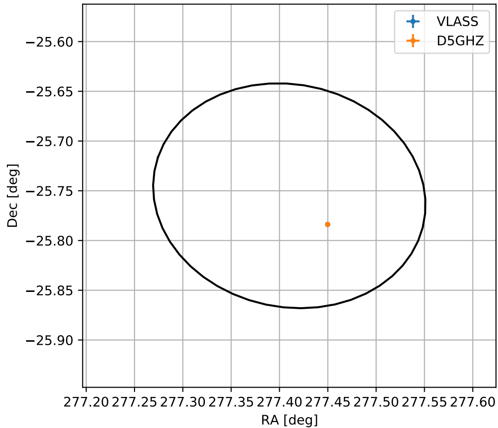
4FGL J1829.6-2545
