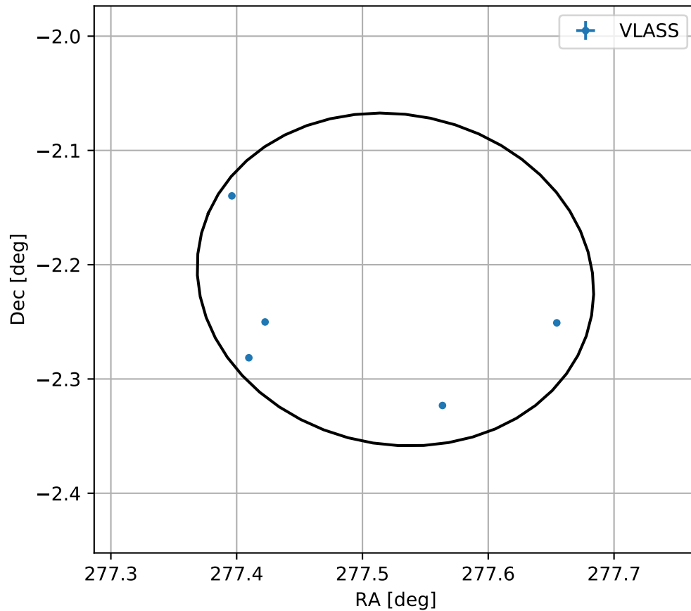
4FGL J1830.1-0212c
