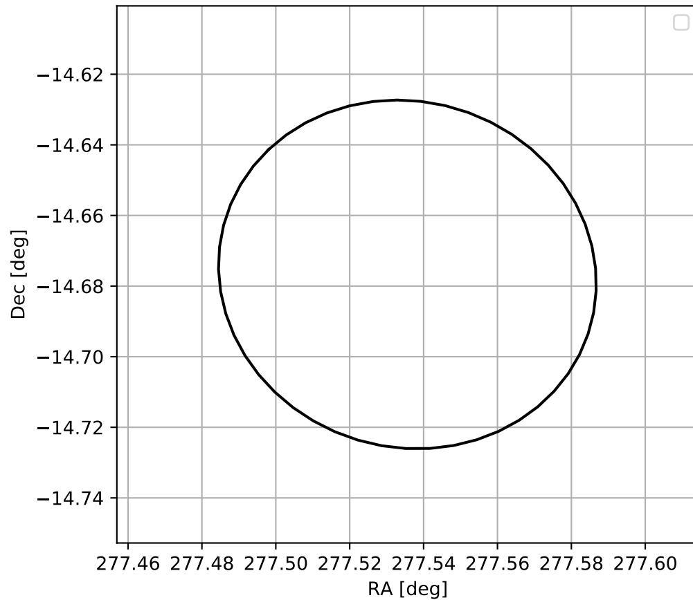
4FGL J1830.1-1440
