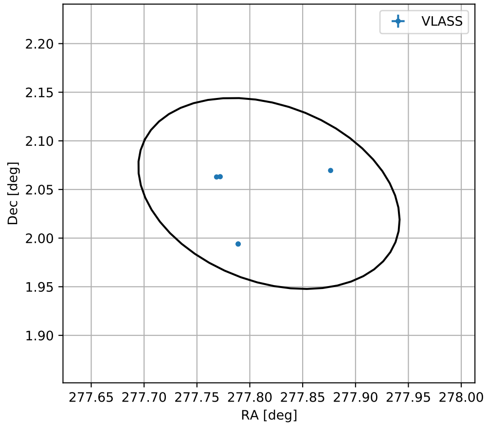
4FGL J1831.2+0202
