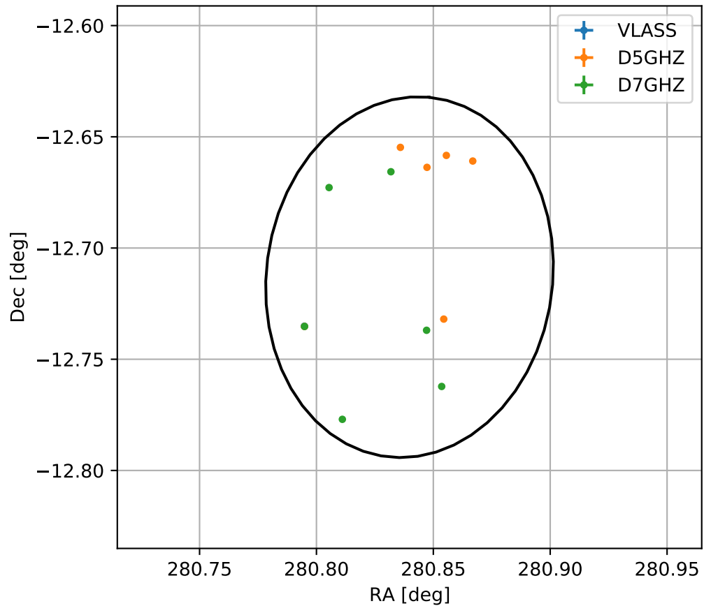
4FGL J1843.3-1242
