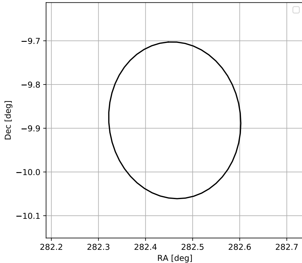
4FGL J1849.8-0952
