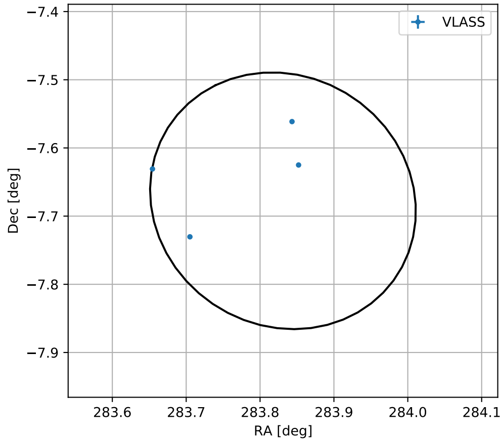
4FGL J1855.3-0740
