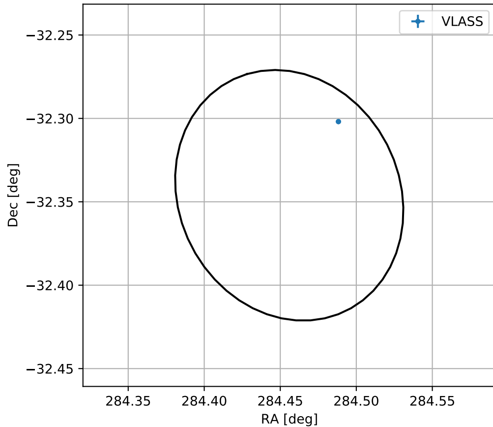
4FGL J1857.8-3220
