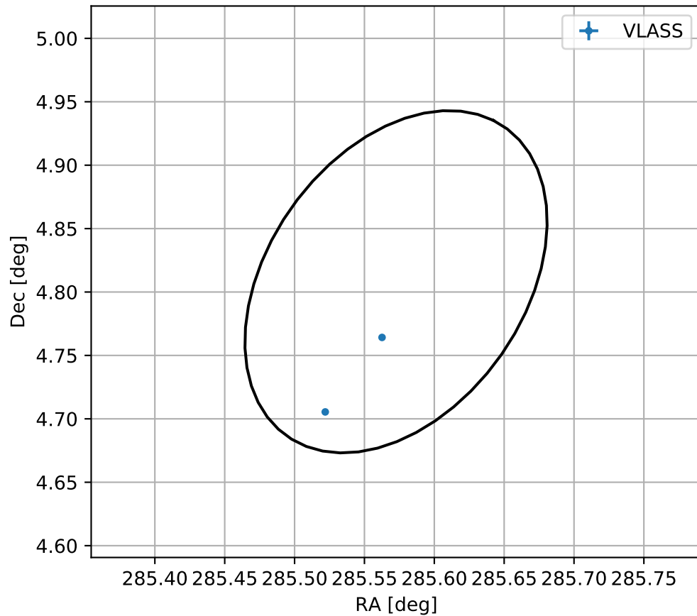
4FGL J1902.2+0448
