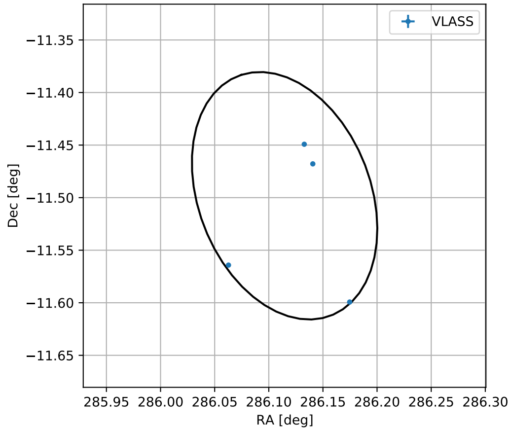
4FGL J1904.4-1129
