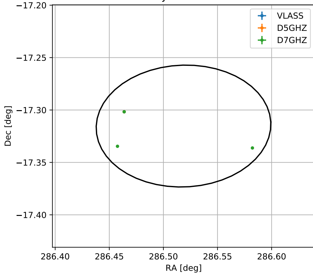
4FGL J1906.0-1718
