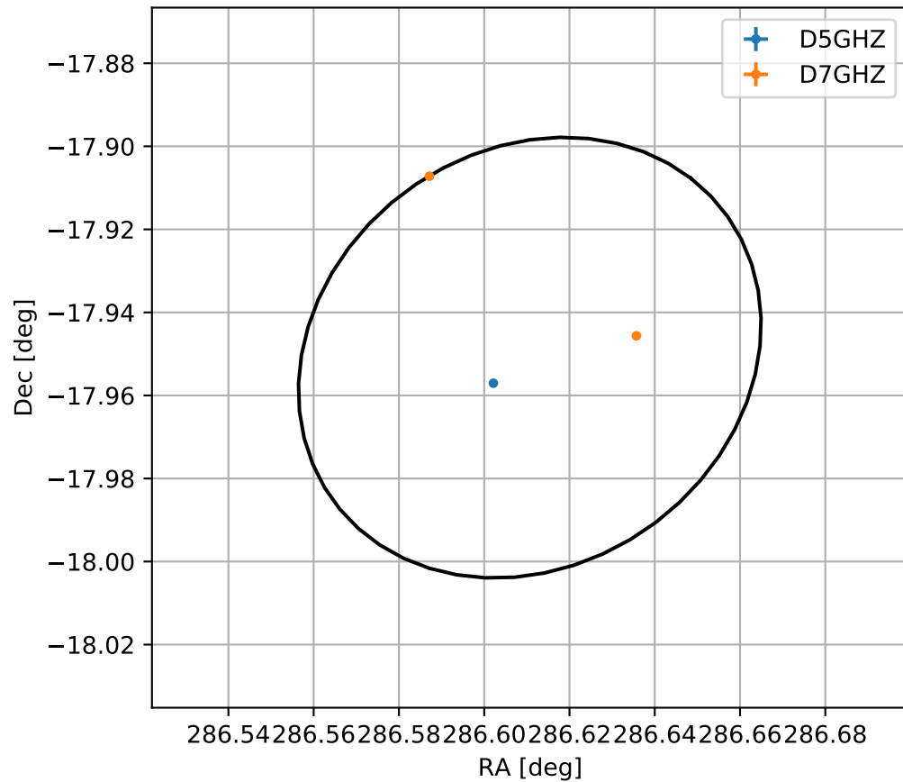
4FGL J1906.4-1757
