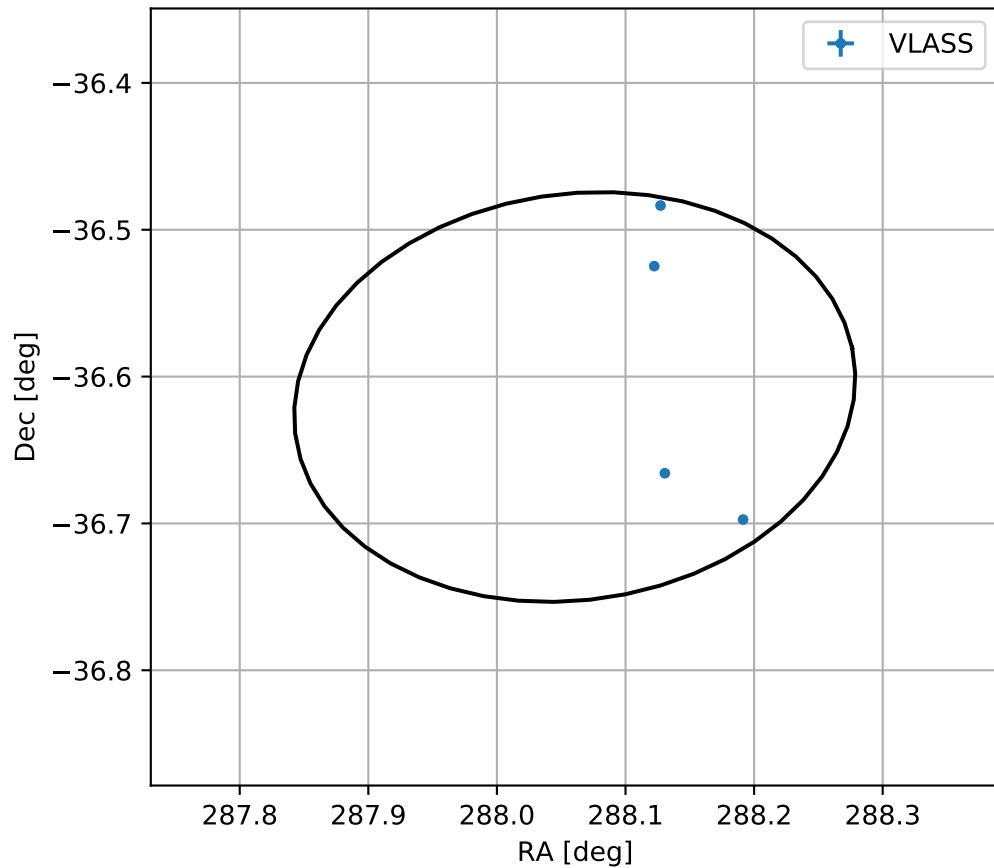
4FGL J1912.2-3636
