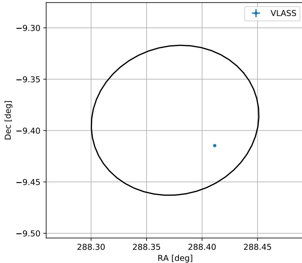
4FGL J1913.5-0923
