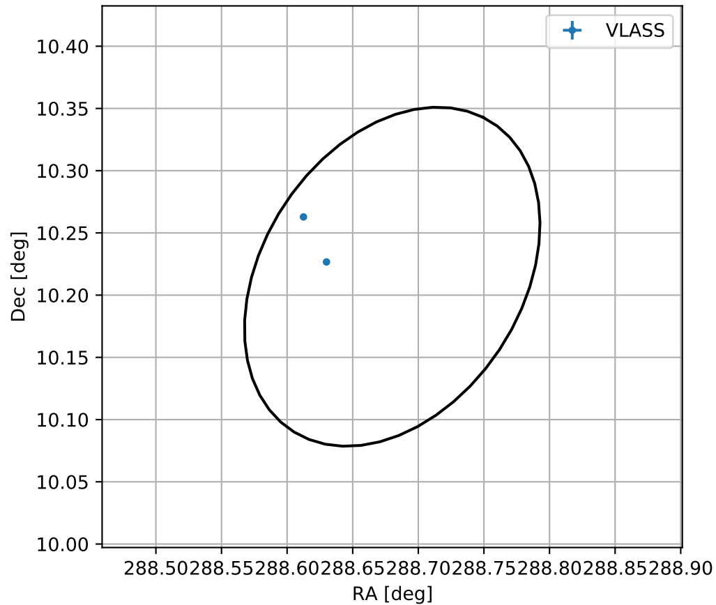
4FGL J1914.7+1012c
