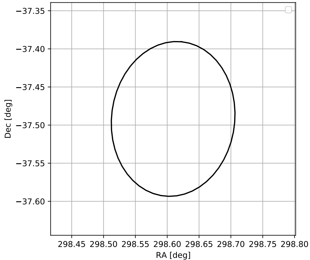
4FGL J1954.4-3729
