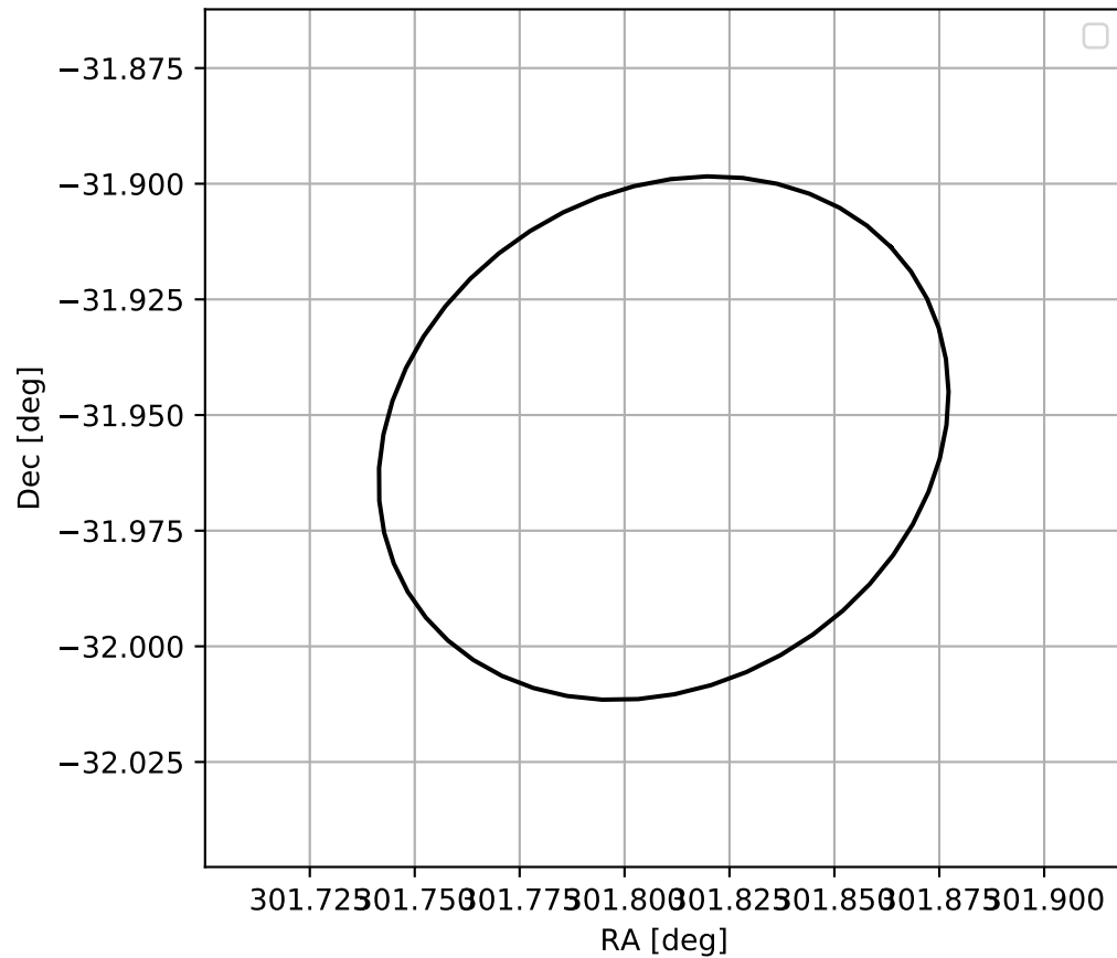
4FGL J2007.2-3157
