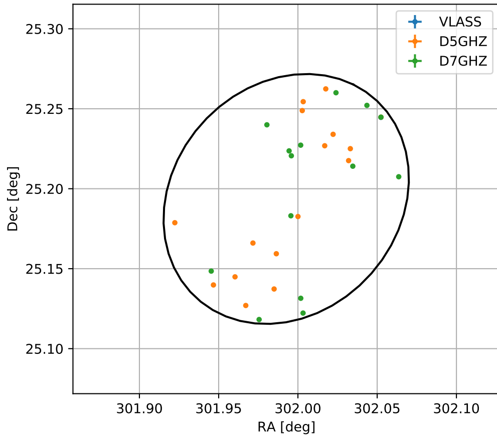
4FGL J2007.9+2511
