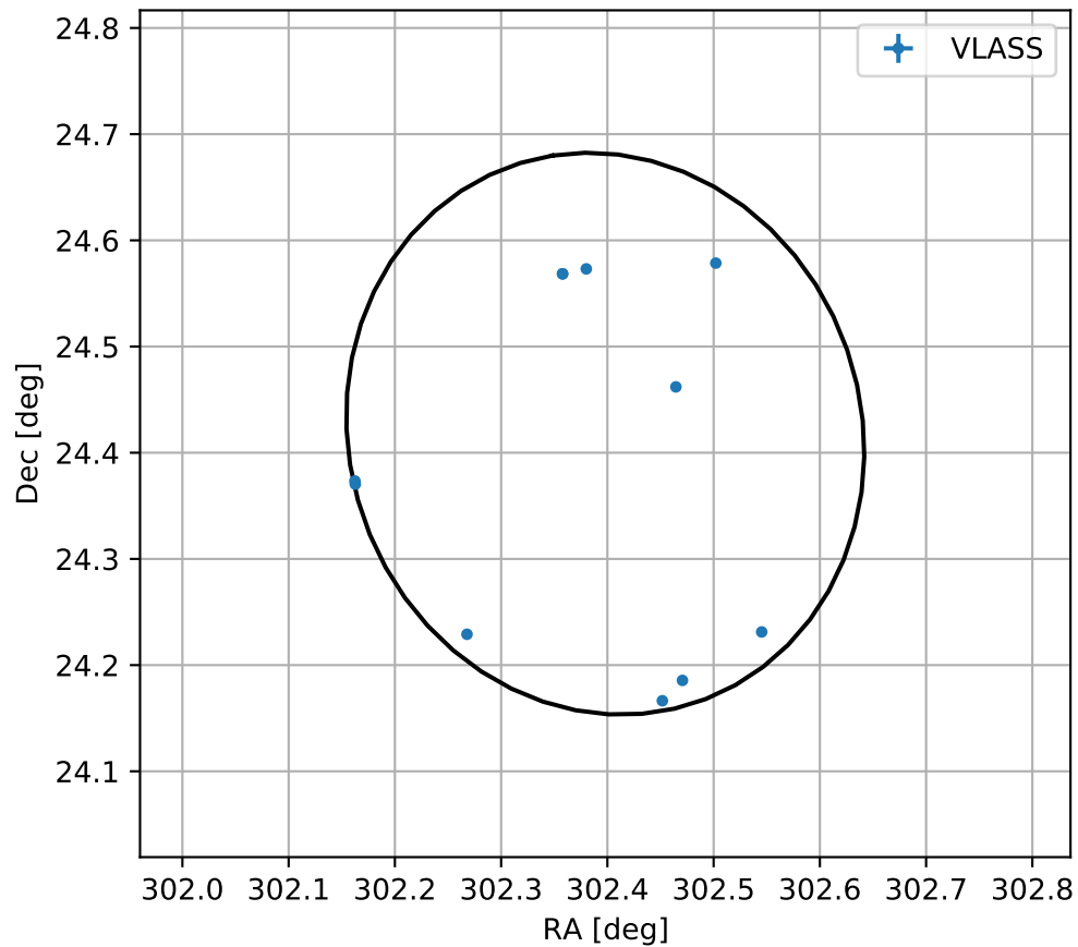
4FGL J2009.5+2425
