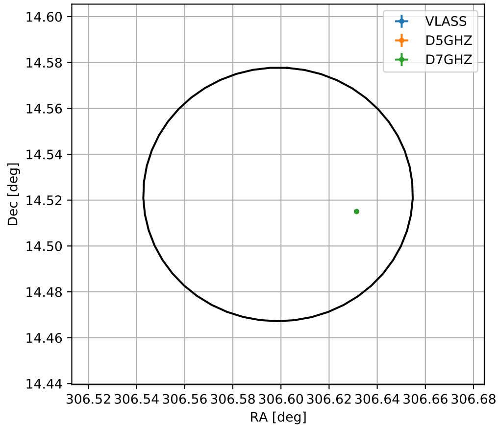
4FGL J2026.3+1431
