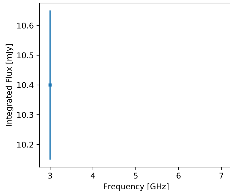
F357 J204027.83+031121.6 (unr)
