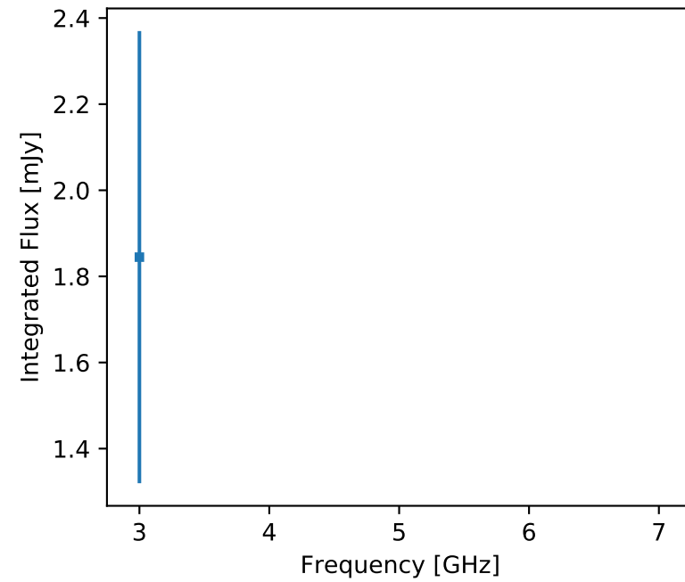
F357 J204027.83+031121.6 (unr)
