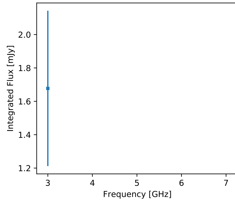
F357 J204018.92+030855.7 (unr)
