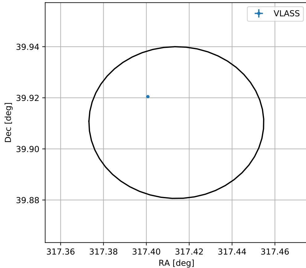
4FGL J2109.6+3954
