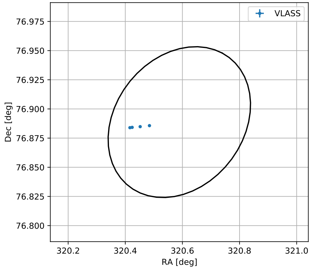
4FGL J2122.3+7653
