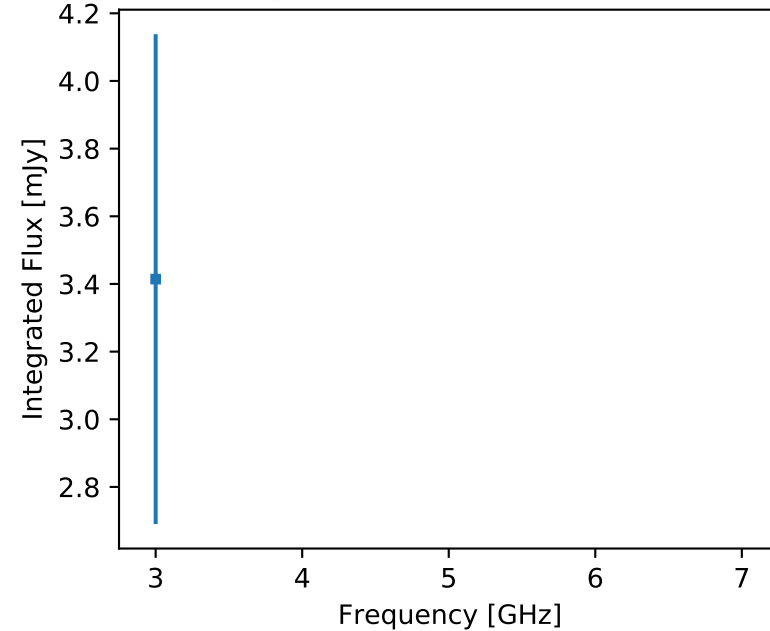
F357 J214718.56-371037.1 (unr)
