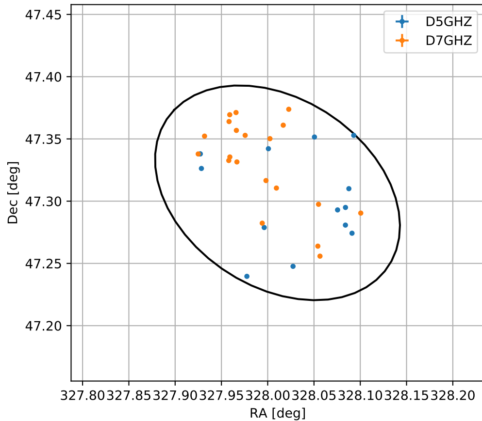
4FGL J2152.0+4718c
