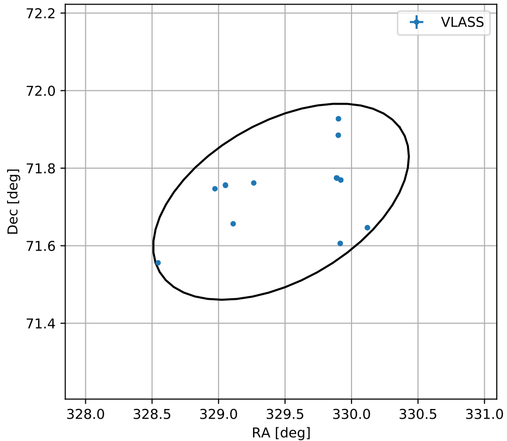
4FGL J2157.8+7142c
