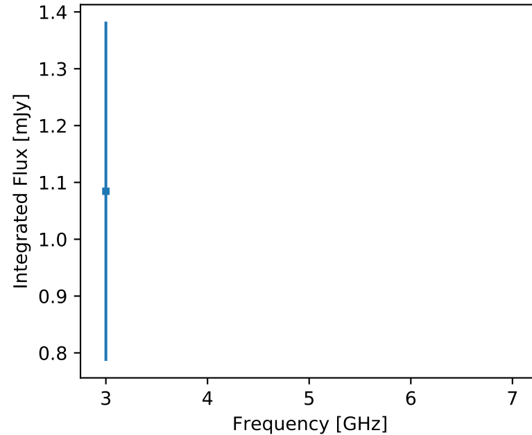
F357 J222856.83+642150.5 (unr)
