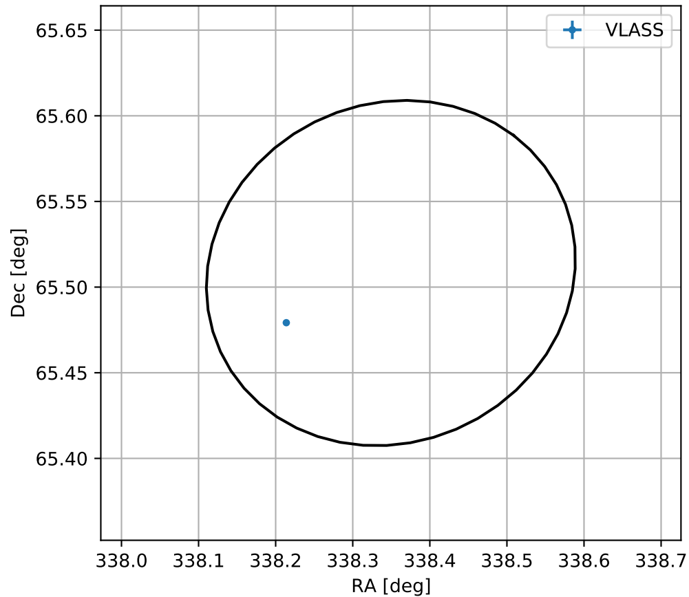
4FGL J2233.3+6530c
