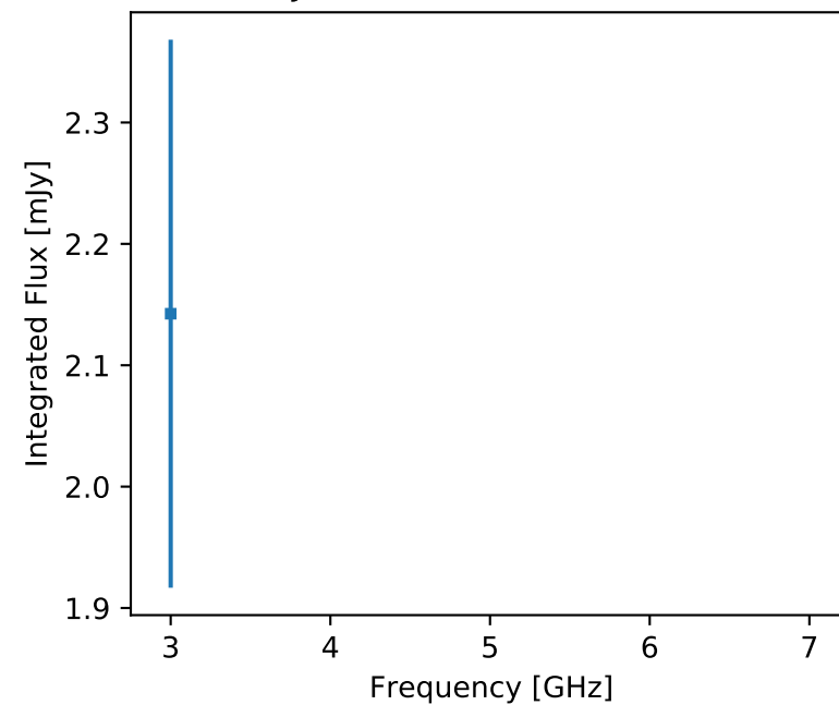
F357 J224129.98+430220.2 (unr)
