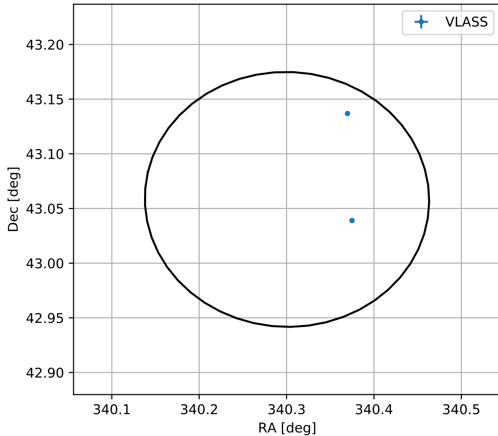
4FGL J2241.2+4303
