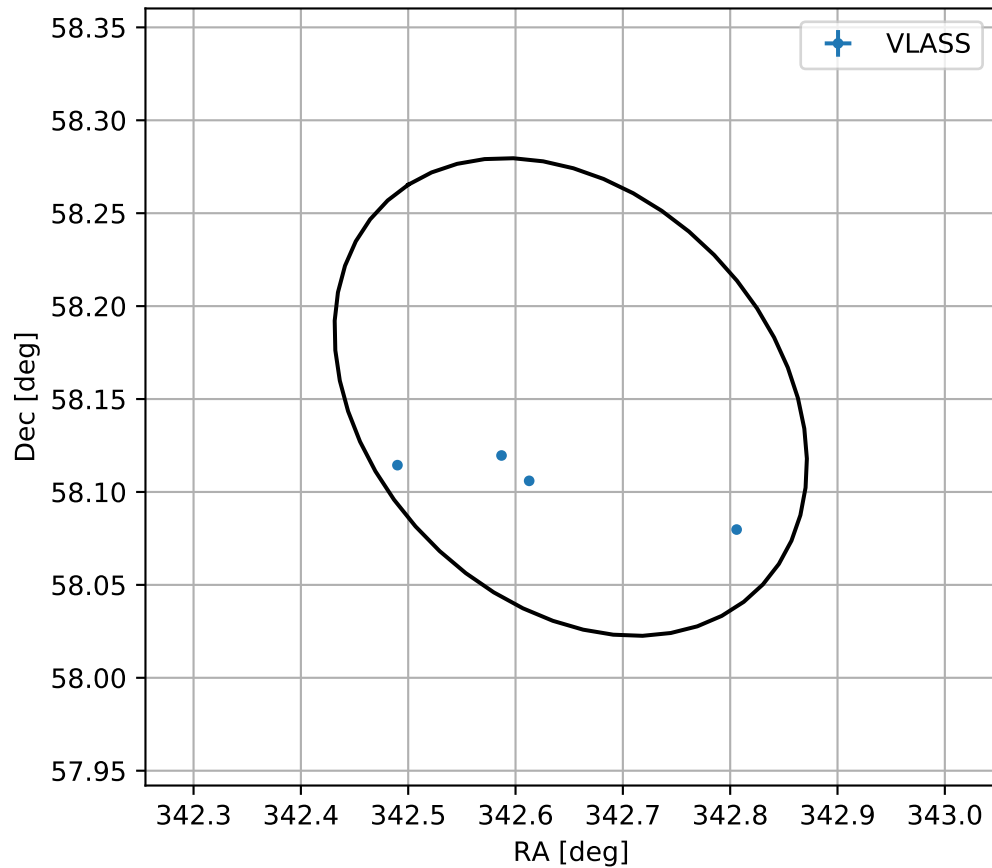
4FGL J2250.6+5809
