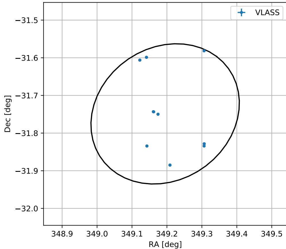
4FGL J2316.7-3144
