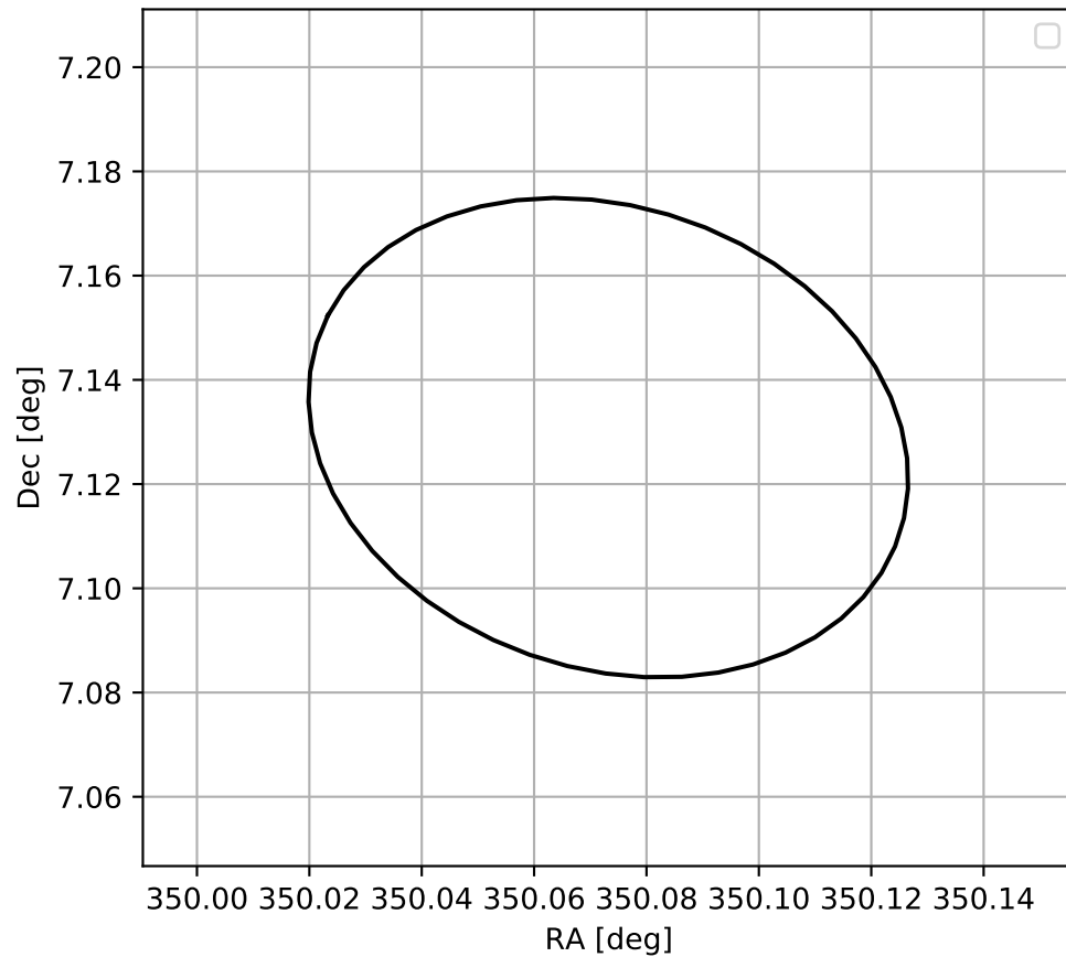
4FGL J2320.2+0707
