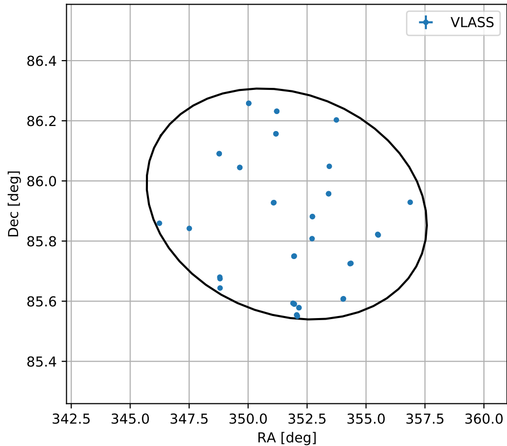
4FGL J2326.5+8555c
