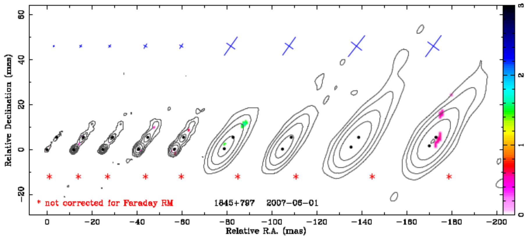
Figure -3.18: Source 1845+797. Faraday-corrected EVPA and linear polarization colour maps in the 1.4 GHz to 15.4 GHz range.
